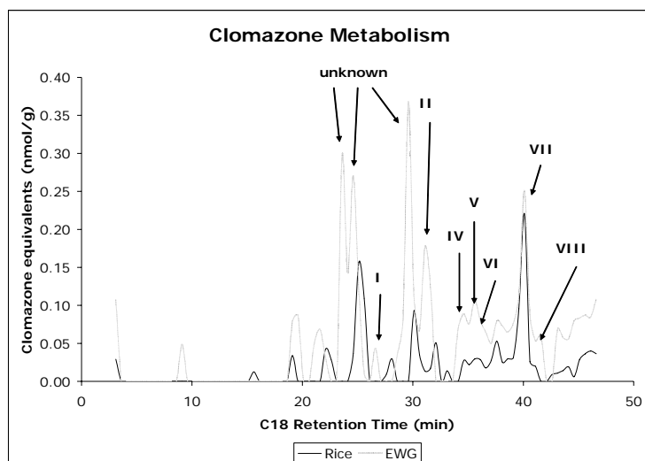
Figure 1. Chromatogram of clomazone and metabolites in rice and early watergrass (EWG). I: 4',5-dihydroxy clomazone; II: 2-chlorobenzoic acid; III: Ring-open reductive product; IV: 3'-hydroxy clomazone; V: 5-hydroxy clomazone; VI: 5'-hydroxy clomazone; VII: clomazone; VIII: 5-ketoclomazone.
