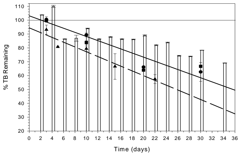
Figure 3. The degradation of thiobencarb in B sterilized soils (vertical bars) and non-sterilized soils with 1.24 mmol Cu(OH) 2 (●), 0.626 mmol CuSO 4 (■) and 21 mmol of PO 4 2- (▲). The solid line is the relative linear regression for both copper treatments (Cu(OH) 2 and CuSO 4 ) while the dashed line is the regression of the phosphate treatment.
