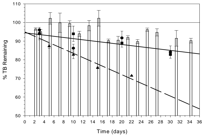
Figure 2. The degradation of thiobencarb in M sterilized soils (vertical bars) and non-sterilized soils with 1.24 mmol Cu(OH) 2 (●), 0.626 mmol CuSO 4 (■) and 21 mmol of PO 4 2- (▲). The solid line is the relative linear regression for both copper treatments (Cu(OH) 2 and CuSO 4 ) while the dashed line is the regression of the phosphate treatment.
