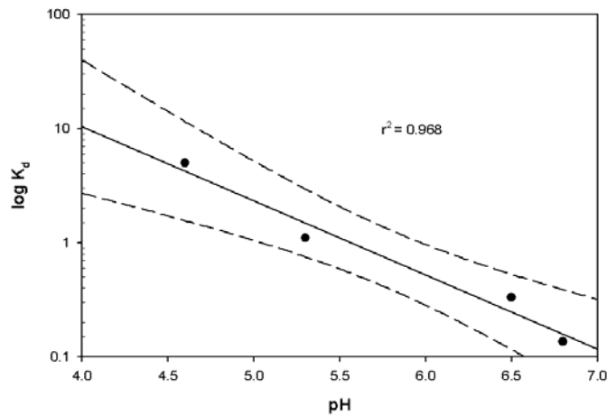
Figure 3. Effect of the soil pH on the Freundlich adsorption coefficient of penoxsulam.
