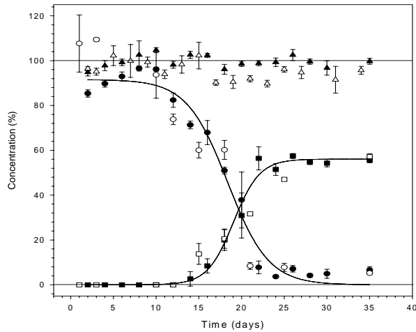
Figure 1. Percent degradation of thiobencarb (97 \mu\text{mol} ) using non-sterile dried ( \bullet ) and permanently wet ( \circ ) soil M and the subsequent formation of deschlorothiobencarb (dried = \blacksquare , permanently wet = \square ). The sterile wet ( \Delta ) and dried ( \blacktriangle ) soils show insignificant loss of thiobencarb over the 35 d sampling period. The solid lines show the logistic degradation and formation for thiobencarb and deschlorothiobencarb in the permanently wet soil, respectively.
