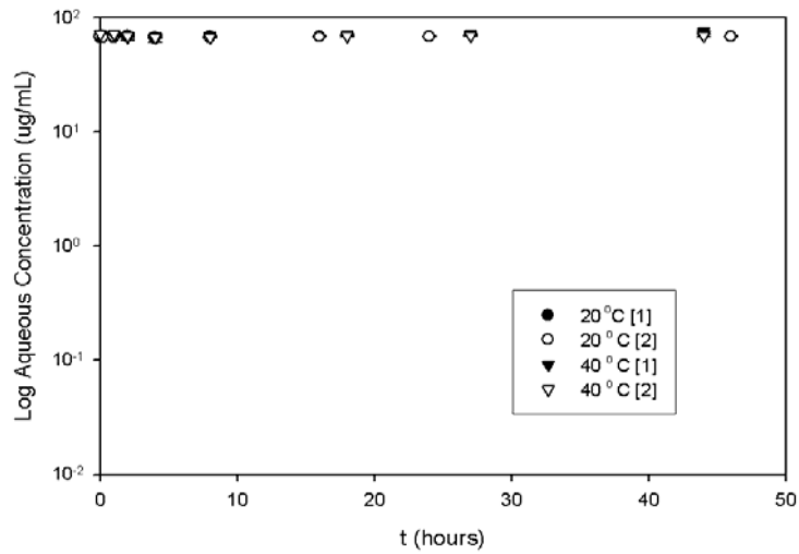
Figure 4. Air-water partitioning of penoxsulam: dissolved concentrations vs. time in the gas-purging experiment.
