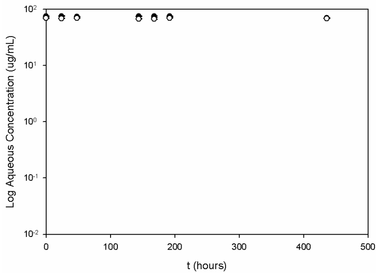
Figure 5. Chemical stability of penoxsulam: dissolved concentrations vs. time in the gas-purging experiment after turning off the gas flow.
