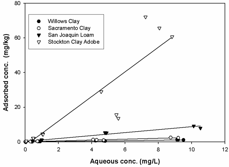
Figure 1. Adsorption of penoxsulam on representative rice field soils of the Sacramento Valley.
