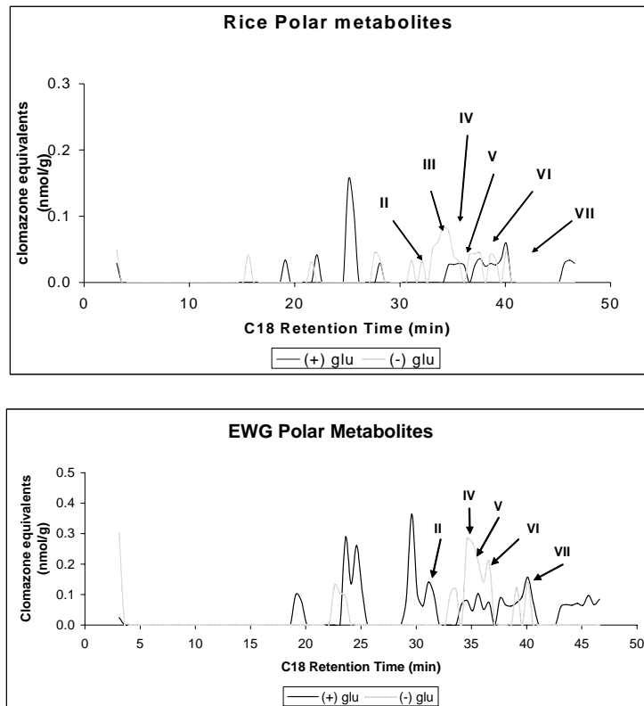
Figure 2. Chromatograms showing polar clomazone metabolites before (+ glu) and after (-glu) treatment with \beta -D-glucosidase in rice (top) and early watergrass (bottom). I: 4',5-dihydroxy clomazone; II: 2-chlorobenzoic acid; III: Ring-open reductive product; IV: 3'-hydroxy clomazone; V: 5-hydroxy clomazone; VI: 5'-hydroxy clomazone; VII: clomazone; VIII: 5-ketoclomazone.
