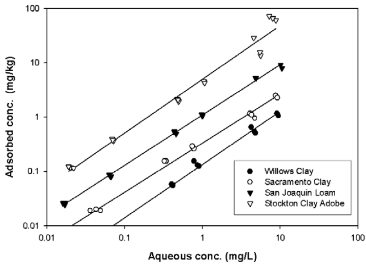
Figure 2. Adsorption of penoxsulam on representative rice field soils of the Sacramento Valley (log-log scale).
